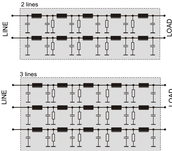
Typical Circuits
