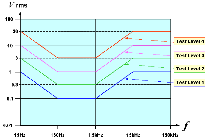
Continuous Test Levels in the range 15Hz to 150kHz (from EN 61000-4-16's Table 3 and figure 2)
