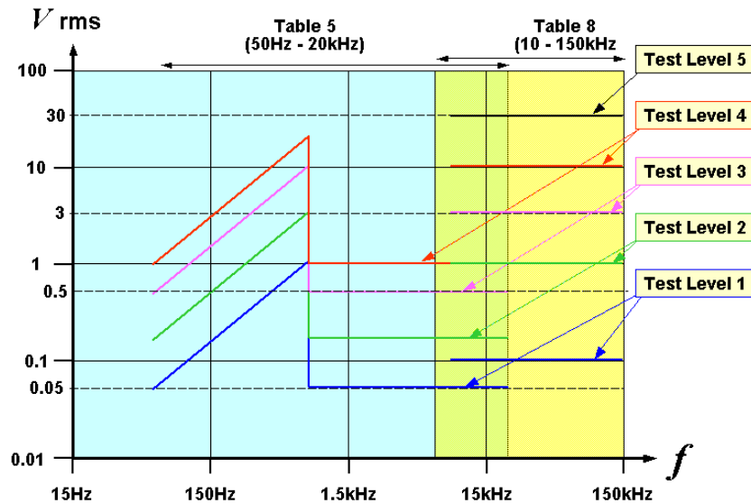
Continuous Test Levels in the range 50Hz to 150kHz (from EN 61000-2-5's Table 5 and 8)
