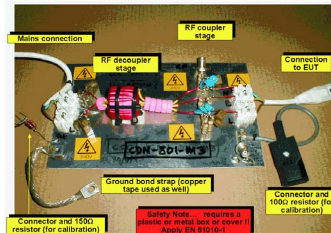
A home-made CDN-M3 (for L,N, E three-wire mains and similar high-voltage cables)
