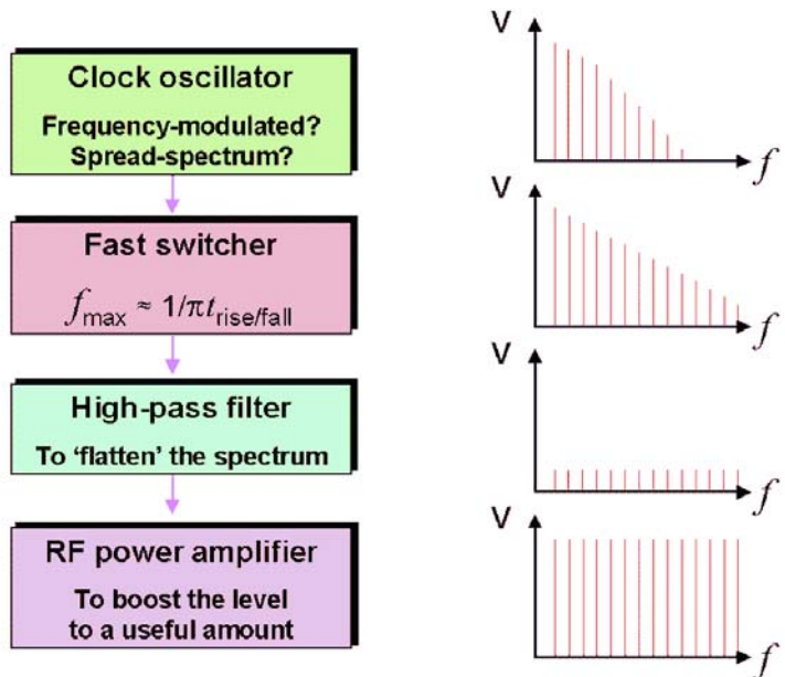
Block diagram of a comb generator
