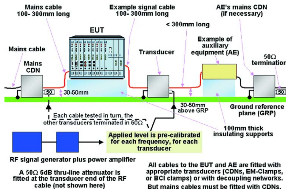
Example of test set-up for EN 61000-4-6
