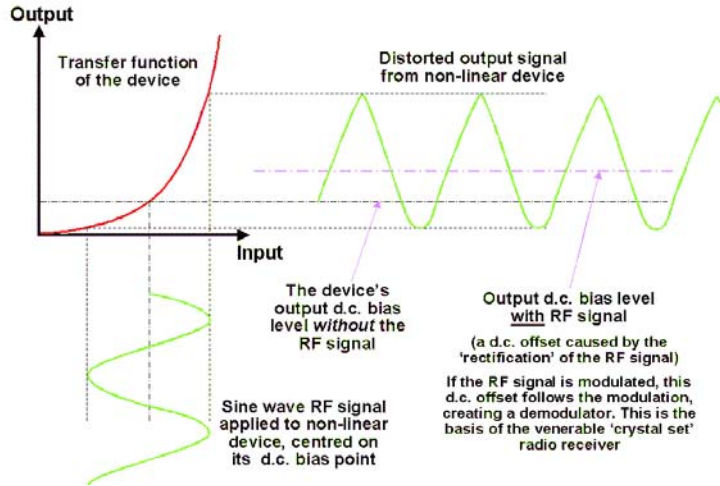
Example of RF noise in a semiconductor circuit showing demodulation and intermodulation
