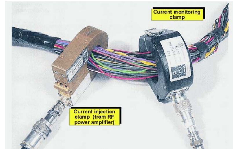
BCI testing a cable bundle (courtesy of the Rover Advanced Technology Centre, Warwick University)
