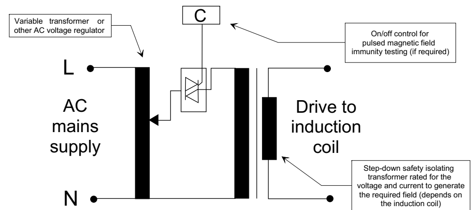
A suitable test generator for EN/IEC 61000-4-8
