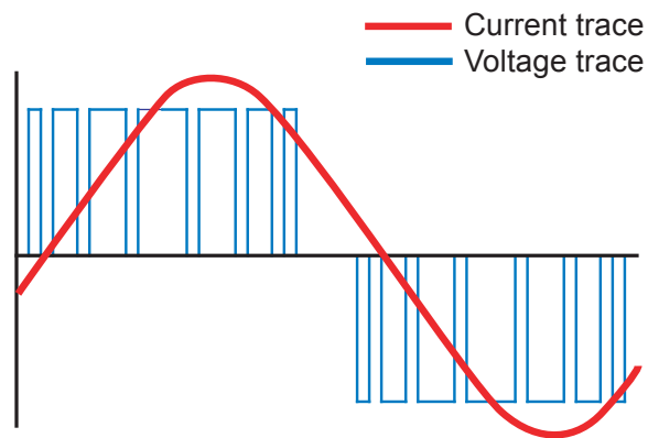
Diagram showing pulse with modulation (switch mode) control
