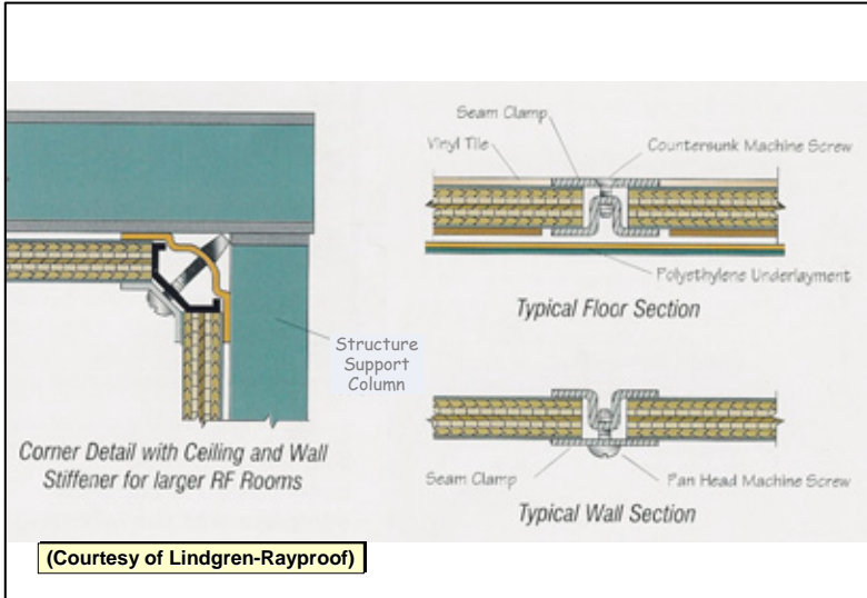
Figure 74 Example of a large shielded room in a facility
