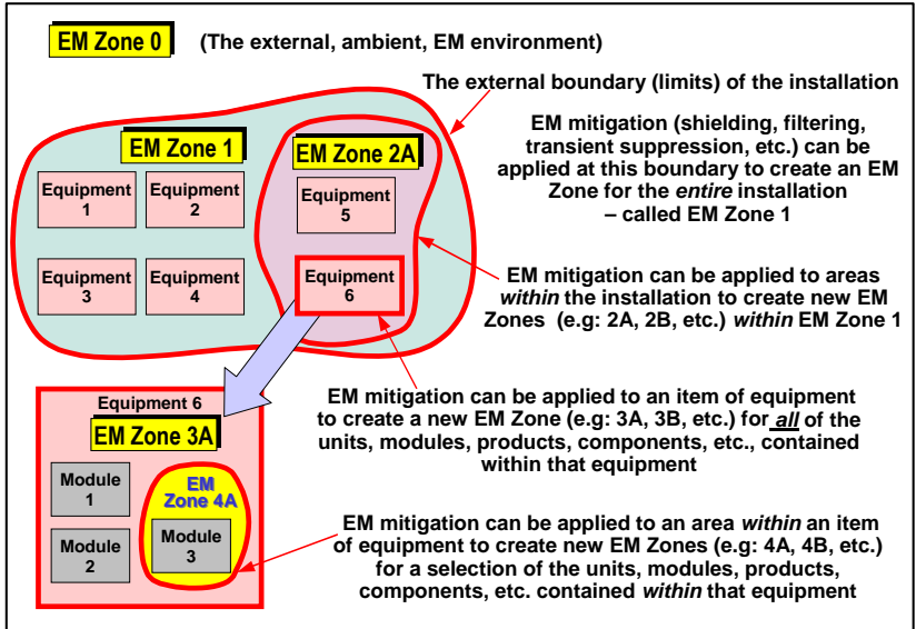
Figure 17 Example of EM Zoning in an installation comprising six items of equipment
