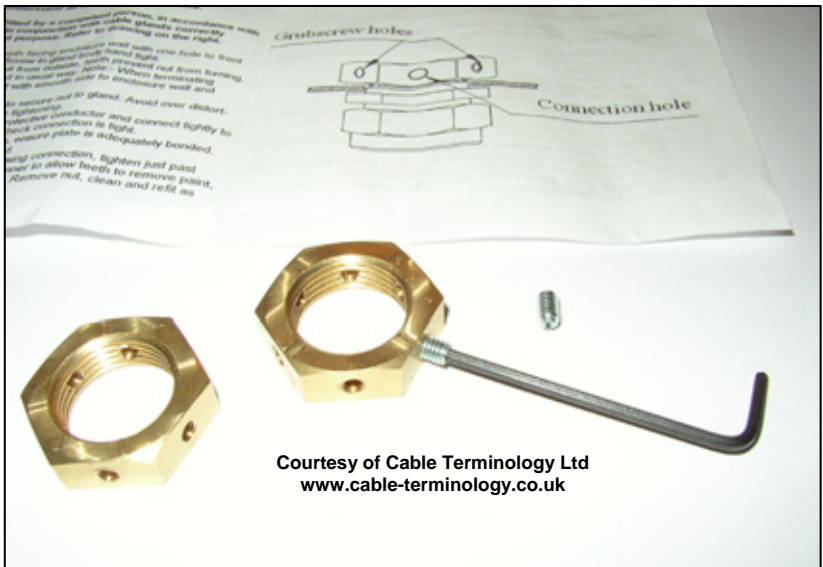
Figure 34 Example of an RF-bonding conduit termination
