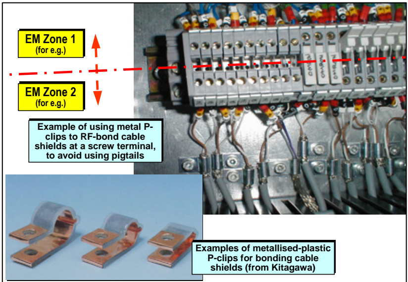
Figure 50 Example of replacing pigtailed cables with P-clips
