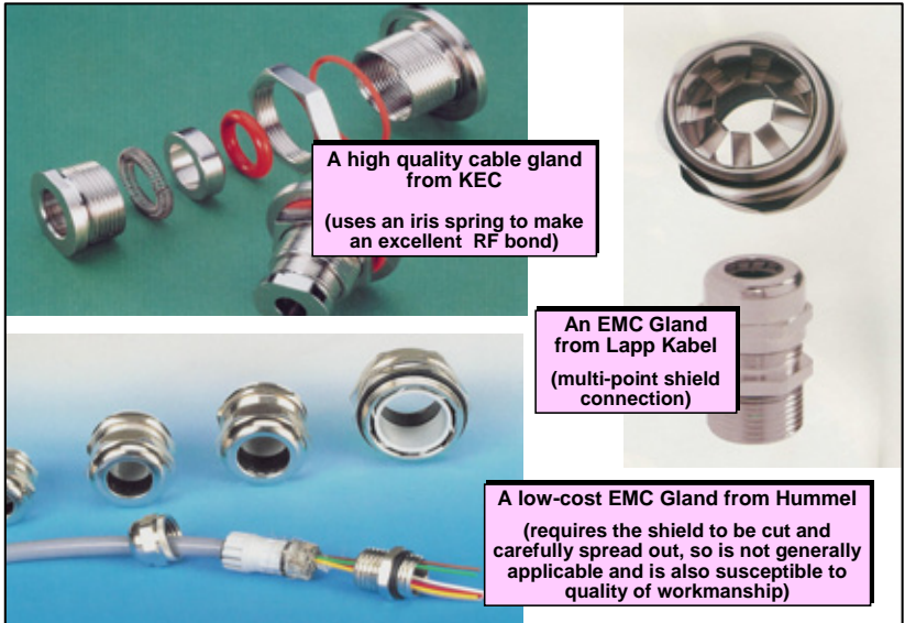
Figure 41 Three types of 360° shielding cable glands ('EMC glands')
