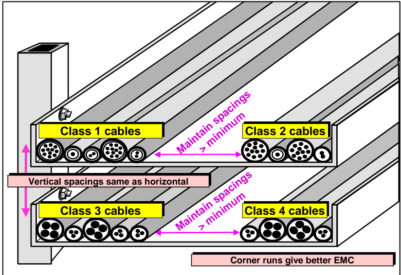
Figure 16 Example of segregating cable Classes in stacked trays
